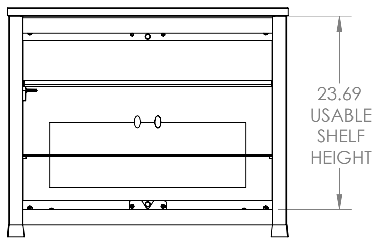
FRONT VIEW WITH DOOR ASSEMBLIES REMOVED
