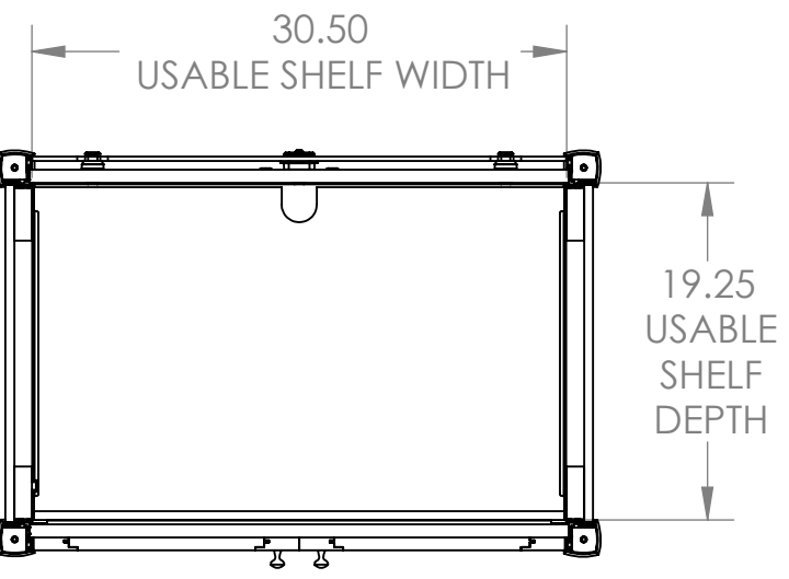
TOP VIEW WITH TOP PANEL REMOVED
