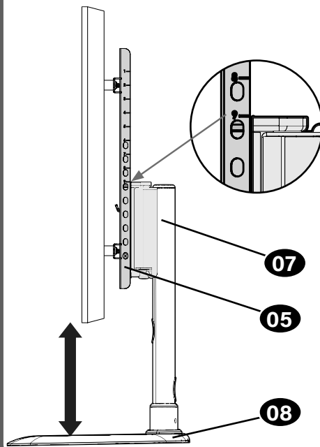
Highest Position
